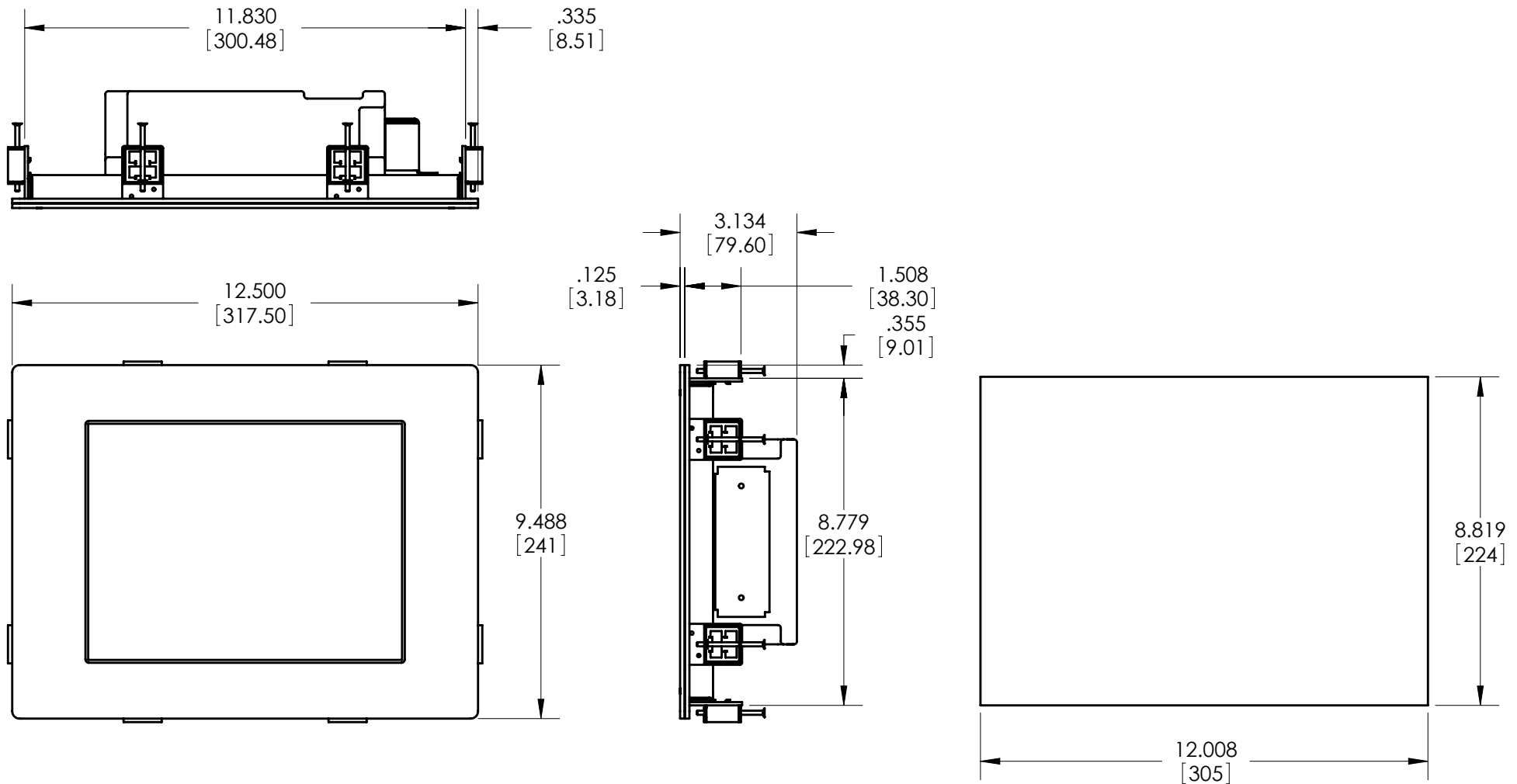
PANEL CUTOUT SIZE
